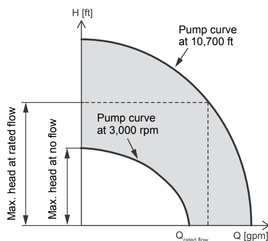
Fig. 14 Recommended sizing
