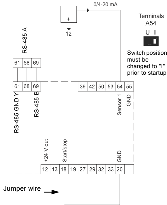
Fig. 36 Wiring diagram for CU331SP
