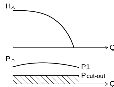
Fig. 1 P_{\text{cut-out}} curve
