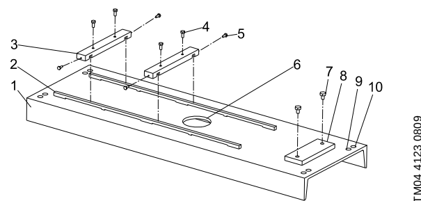
Fig. 11 Plaque de support Grundfos
