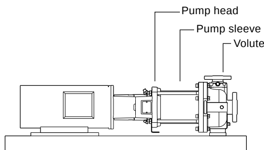
Fig. 12 Potentially hot surfaces on a CR-H and CRN-H pump
