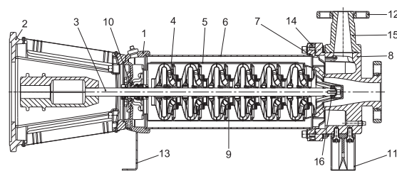
Fig. 20 Sectional drawing
