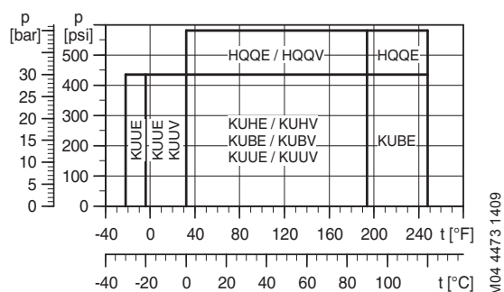
Fig. 22 Operating range of standard shaft seals for CR(E), CRN(E) 32 H to CR 90 H
