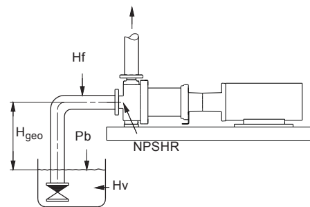
Fig. 24 Sizing data
