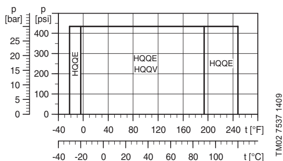
Fig. 21 Operating range of standard shaft seals for CR(E), CRN(E) 1s H to CR 20 H
