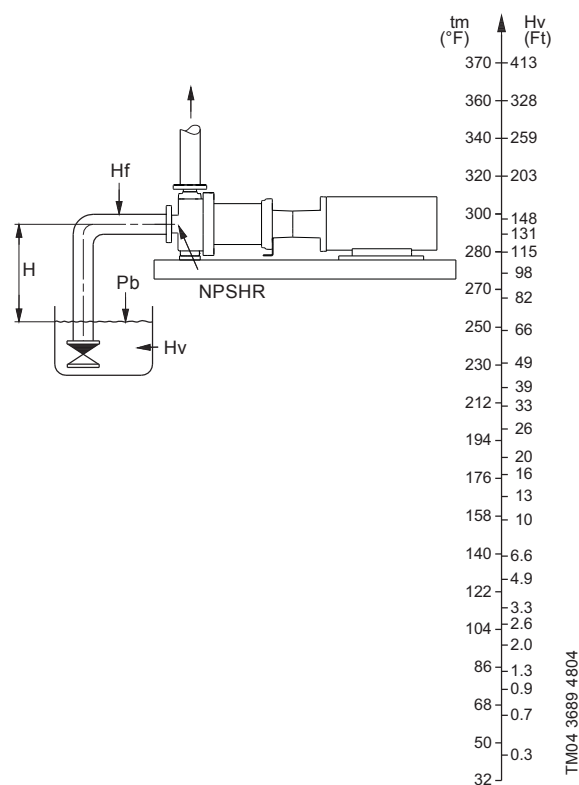
Fig. 32 Minimum inlet pressure - NPSHR
