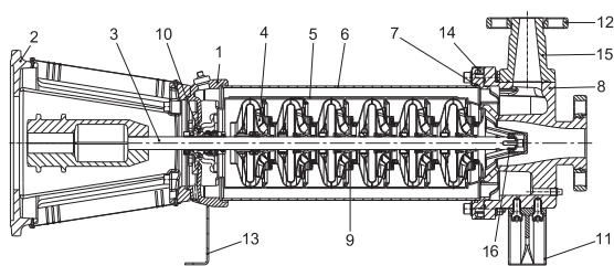
Fig. 18 Sectional drawing
