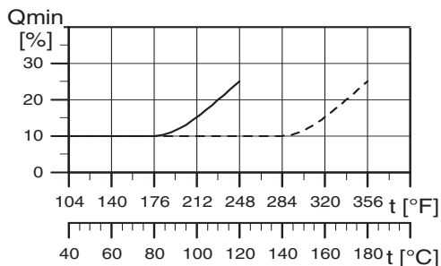
Fig. 34 Minimum flow rate
