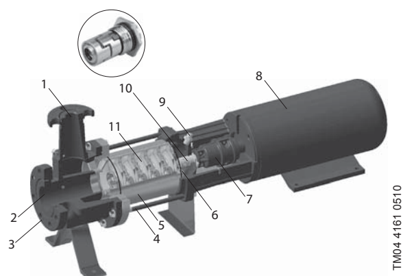
Fig. 2 CR-H pump
