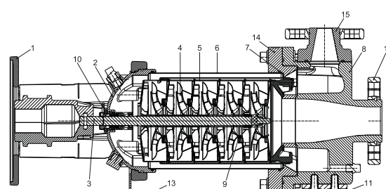
Fig. 16 Sectional drawing
