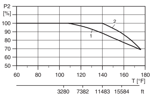
Fig. 4 Relationship between motor output ( P_2 ) and ambient temperature/altitude
