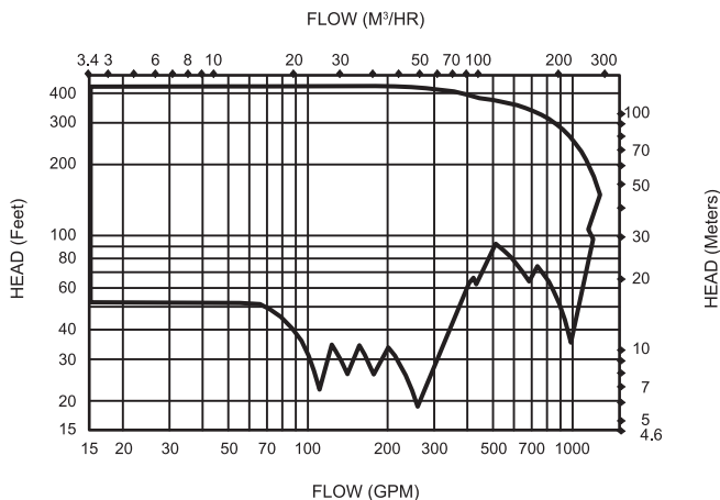
C Series Range Chart - 3500 RPM
