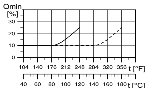
Fig. 28 Minimum flow rate
