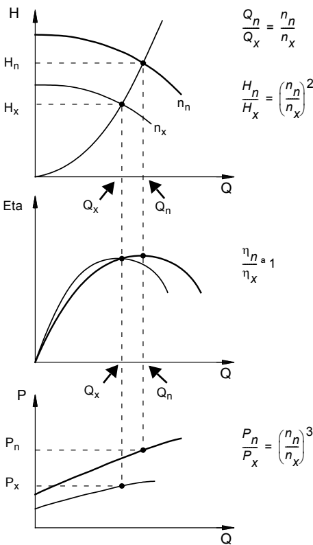
Fig. 22 Affinity equations
