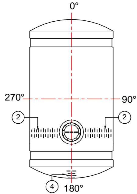
PLAN VIEW
